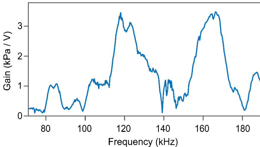
Figure S2. The measured transfer function (TF) produced pressure as a result of input voltage. The gain of the TF, which is the pressure produced by the transducer vs. input voltage is plotted as a function of the frequency. The TF captures the dynamics of the transducer, glass slide, and peripheral electronics. Large TF values indicate optimal excitation frequencies.
